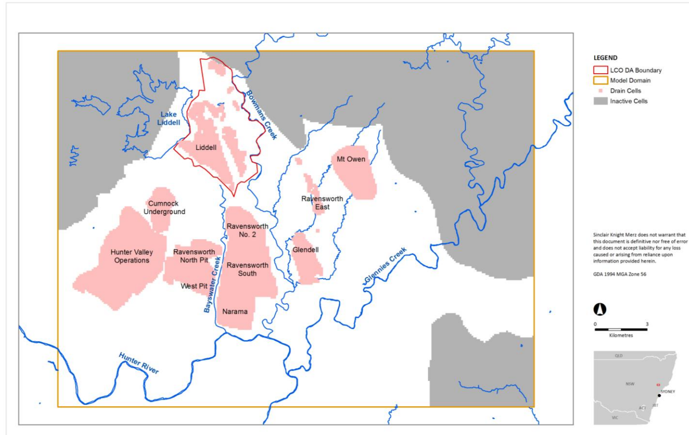
Figure B-8 – Model Drain Cells for Layer 4
