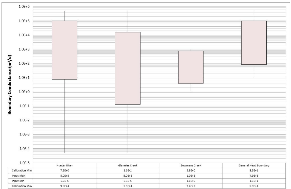
■ Figure 3-10 – Model Parameter Sensitivity: Boundary Conductance
