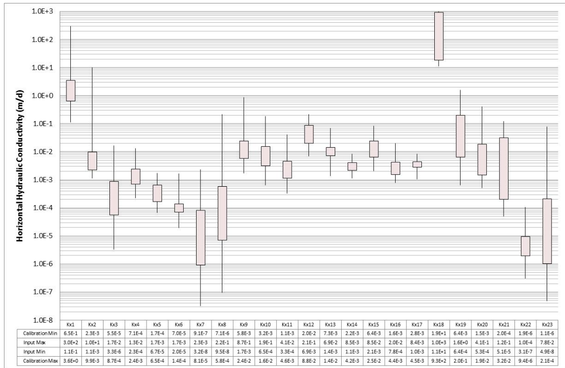
■ Figure 3-7 – Model Parameter Sensitivity: Horizontal Hydraulic Conductivity
