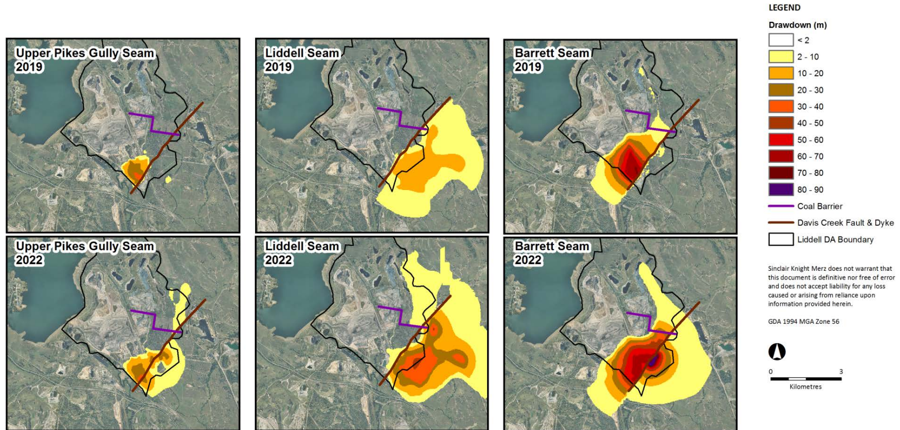
Figure 3-17 – Predicted Drawdown for Coal Seams Resulting from Proposed Modification
