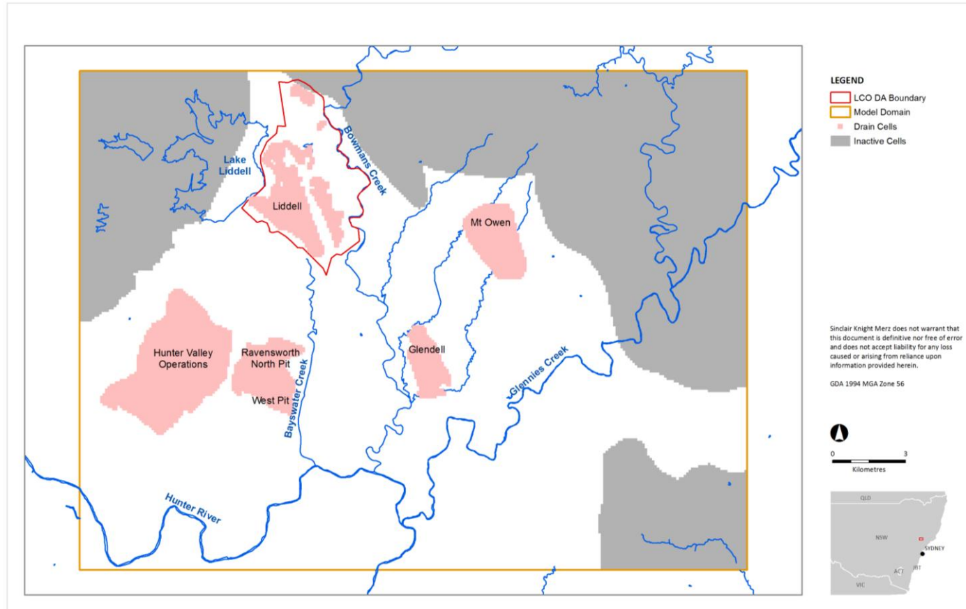
Figure B-16 – Model Drain Cells for Layer 12
