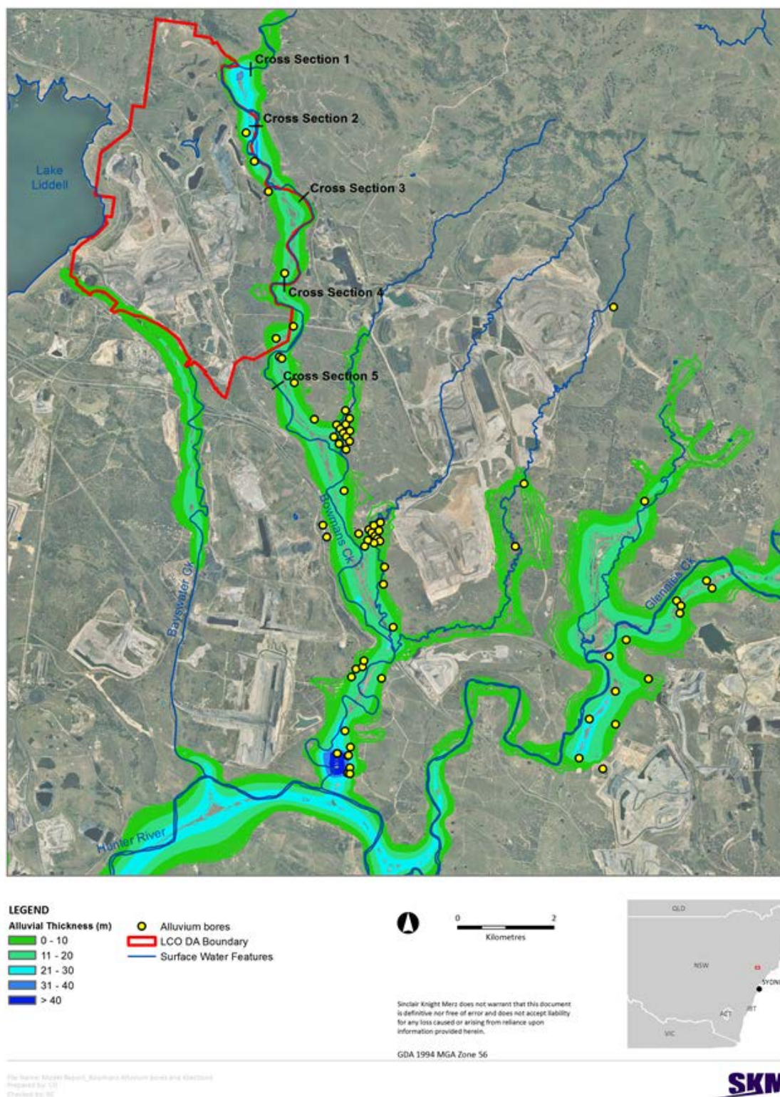
■ Figure 2-11 – Extent of Bowmans Creek Alluvial Aquifer within the Model
