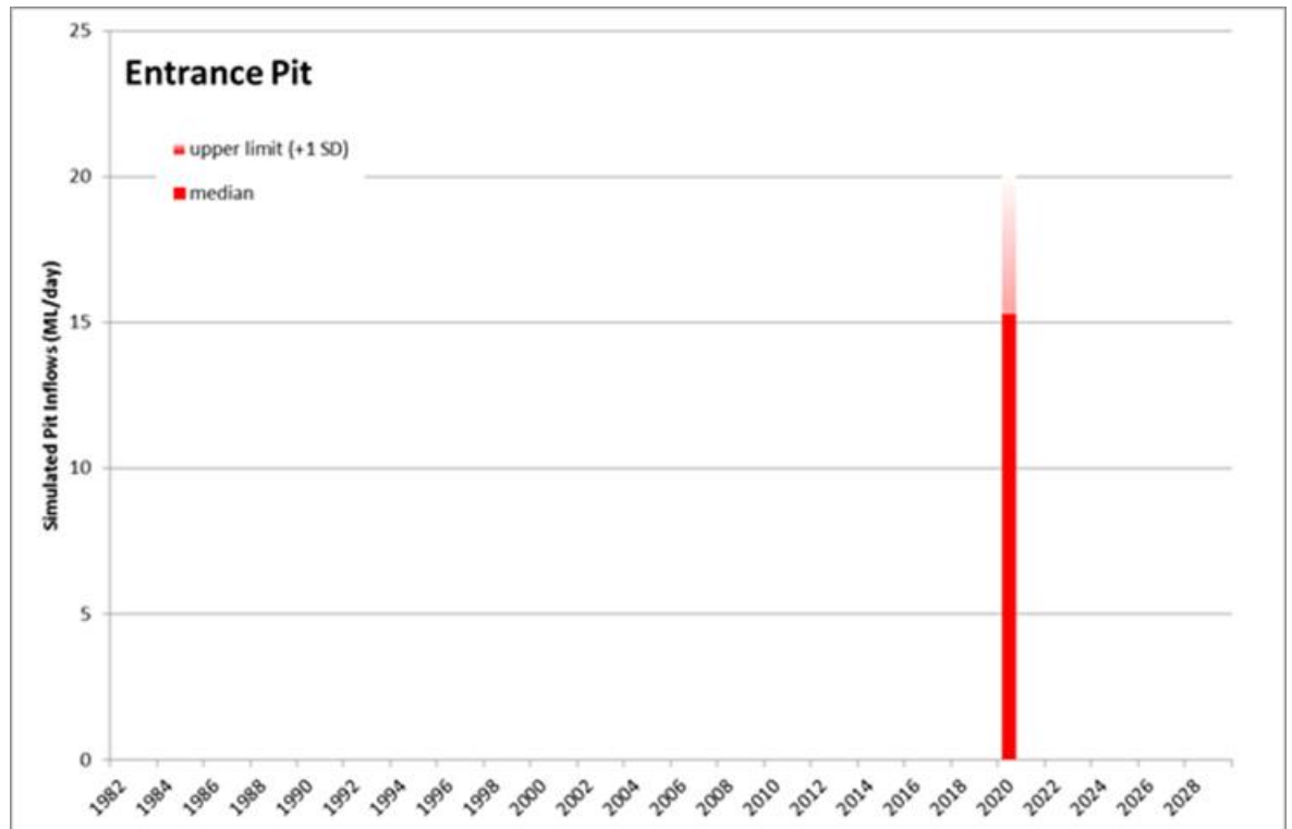
■ Figure 3-19 – Estimated Pit Inflows at Entrance Pit
