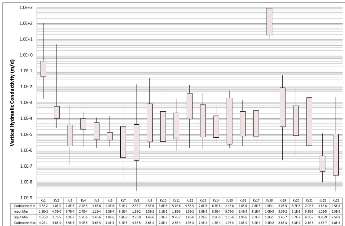
■ Figure 3-8 – Model Parameter Sensitivity: Vertical Hydraulic Conductivity
