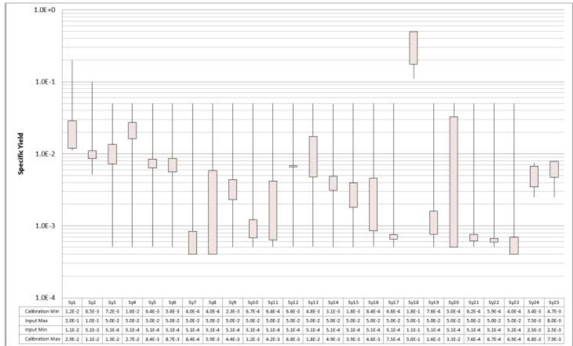
■ Figure 3-9 – Model Parameter Sensitivity: Specific Yield
