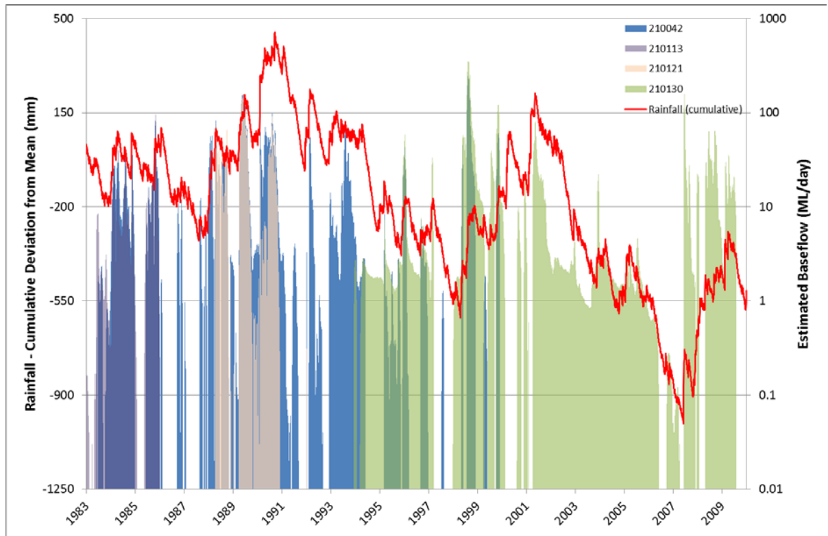
■ Figure 2-6 – Estimated Baseflow Contributions and Rainfall for Bowmans Creek
