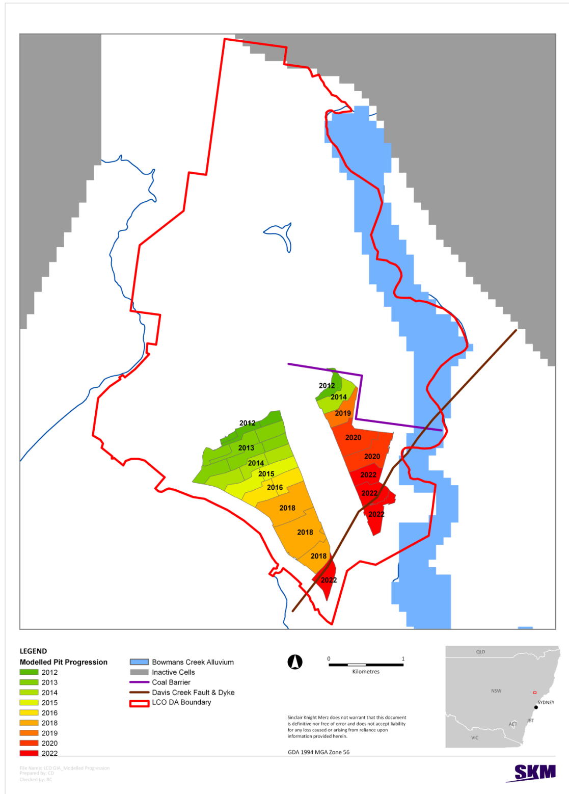
■ Figure 3-13 – Modelled Open Pit Progression for Proposed Case Scenario
