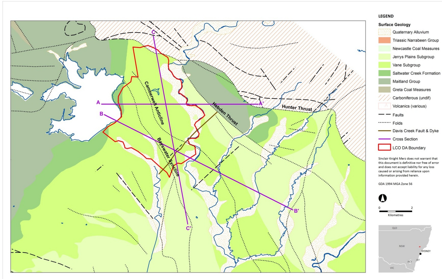
■ Figure 2-7 – Regional Geology and Structural Features
