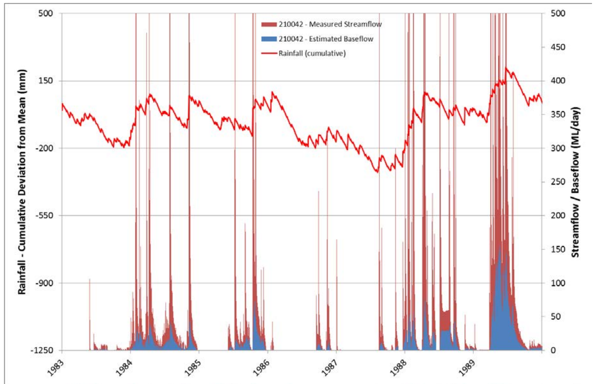
■ Figure 2-17 – Streamflow and Estimated Baseflow Data for Gauge 210042
