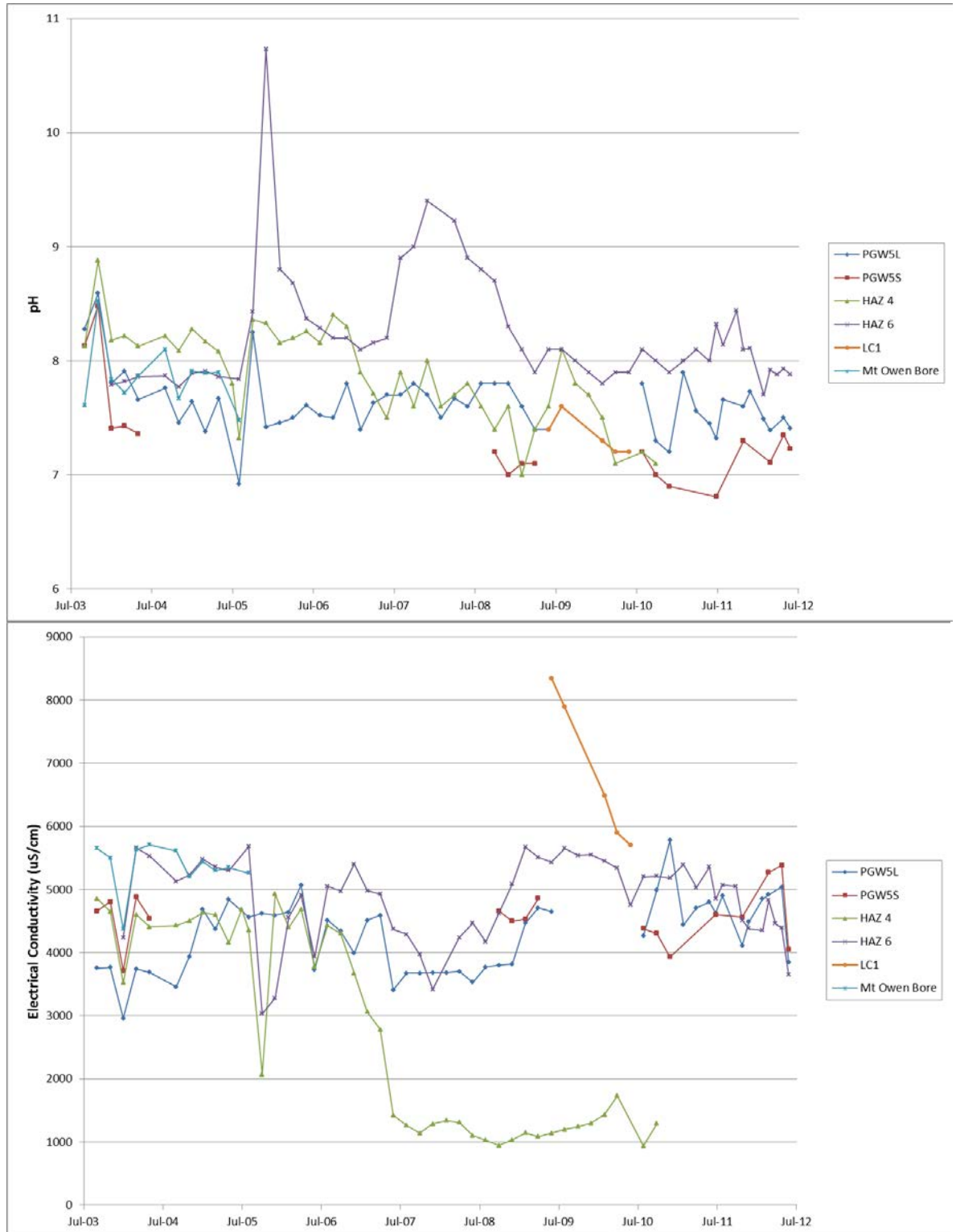
■ Figure 2-20 – pH and Conductivity Data for Piezometers Targeting Regional Hard Rock Aquifer (Coal Measures)
