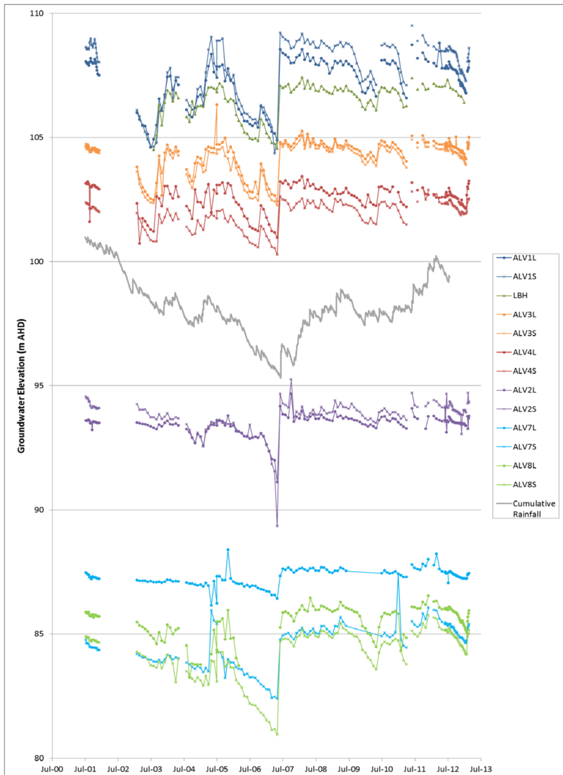
■ Figure 2-14 – Hydrographs for Piezometers Targeting Alluvium and Shallow Bedrock
