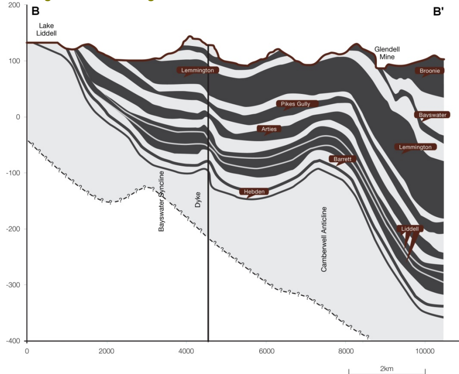
■ Figure 2-9 – Geologic Cross Section B – B'
