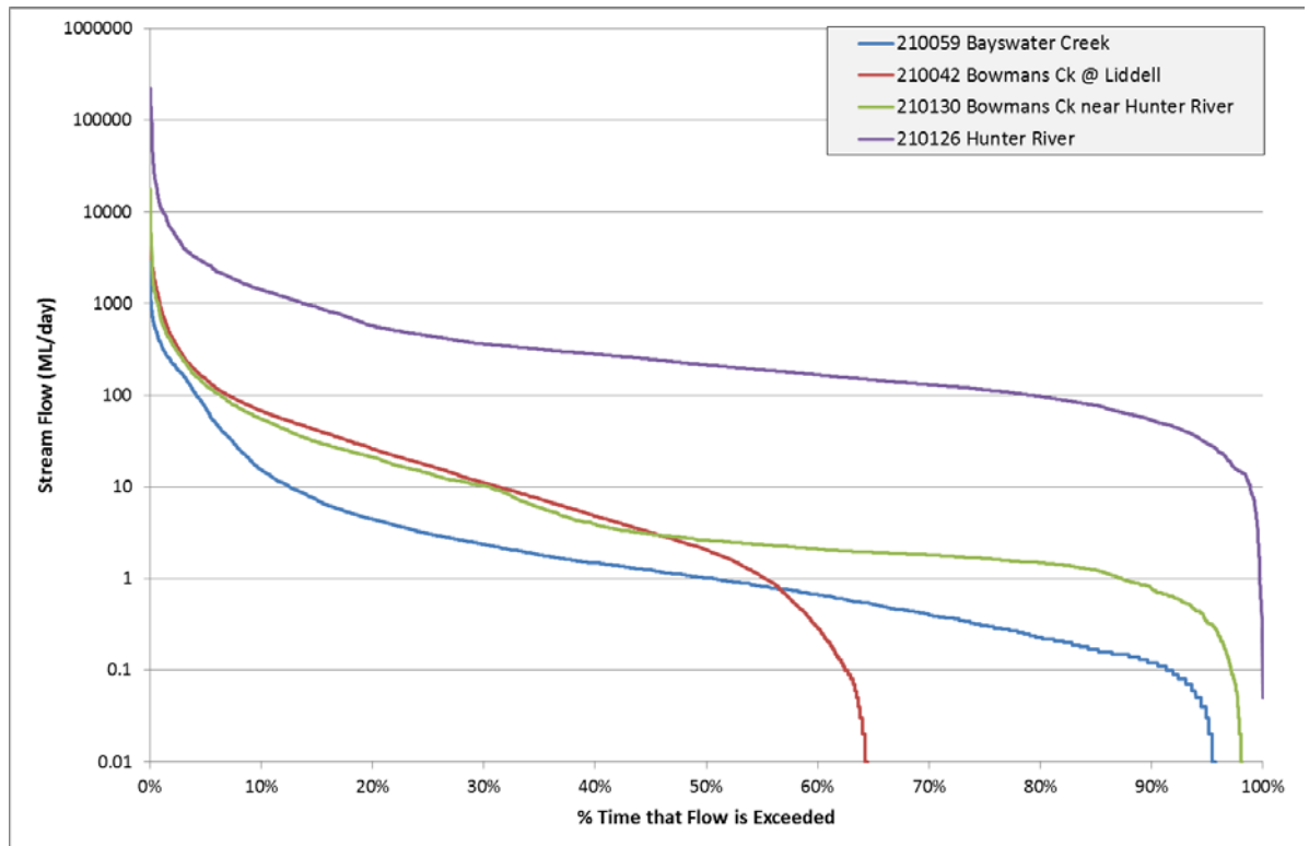
■ Figure 2-5 – Flow Duration Curves for Surface Water Features
