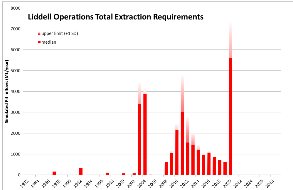
■ Figure 3-20 – Total Estimated Groundwater Extraction Requirements
