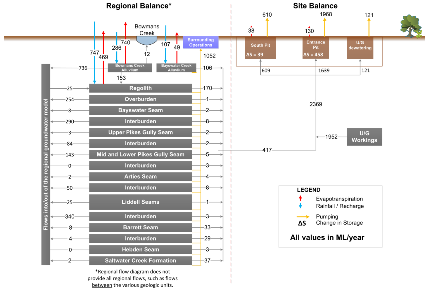
• Figure 3-24 - Modelled regional and local water balance for LCO in Year 9 (approximately 2022)
