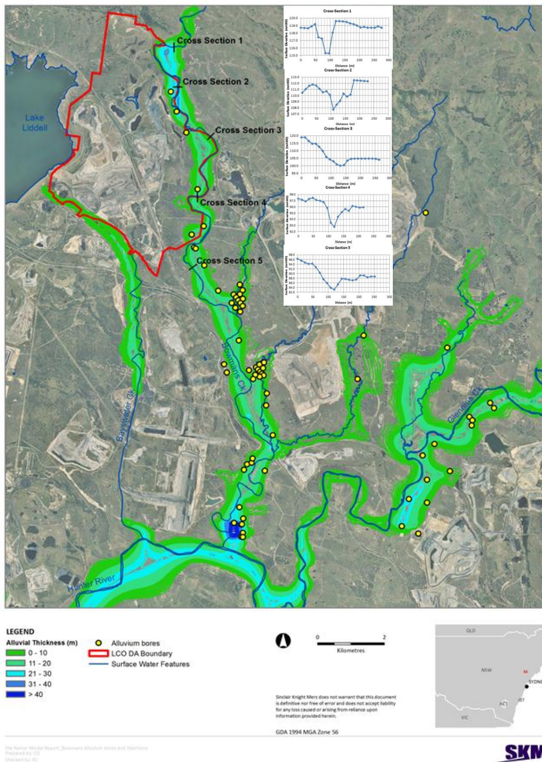
Figure B-2 – Modelled Thickness and Extent of Alluvium
