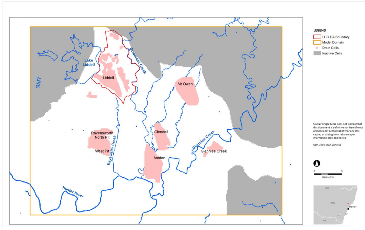
Figure B-21 – Model Drain Cells for Layer 17
