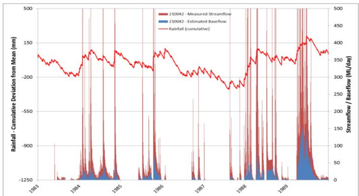
• Figure 2-2 – Measured streamflow and calculated baseflow adjacent to the Liddell mining lease and cumulative rainfall deviation curve
