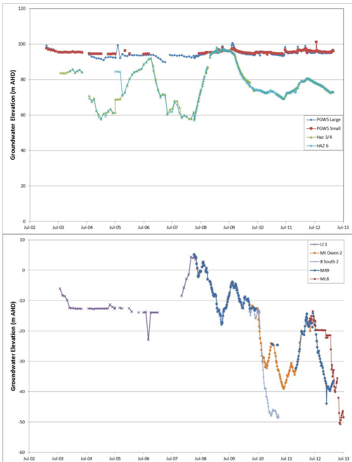
■ Figure 2-16 – Hydrographs for Piezometers Targeting Regional Hard Rock Aquifer (Coal Measures)
