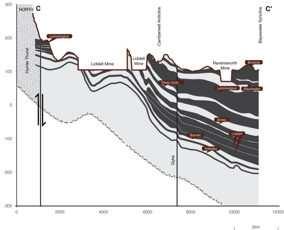
■ Figure 2-10 – Geologic Cross Section C – C'
