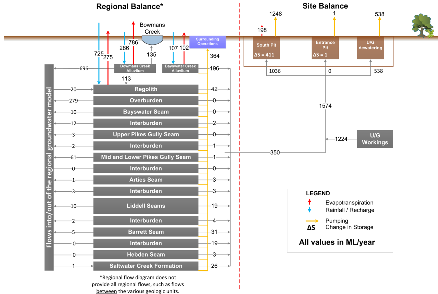
Figure 3-23 - Modelled regional and local water balance for LCO in Year 5 (approximately 2018)
