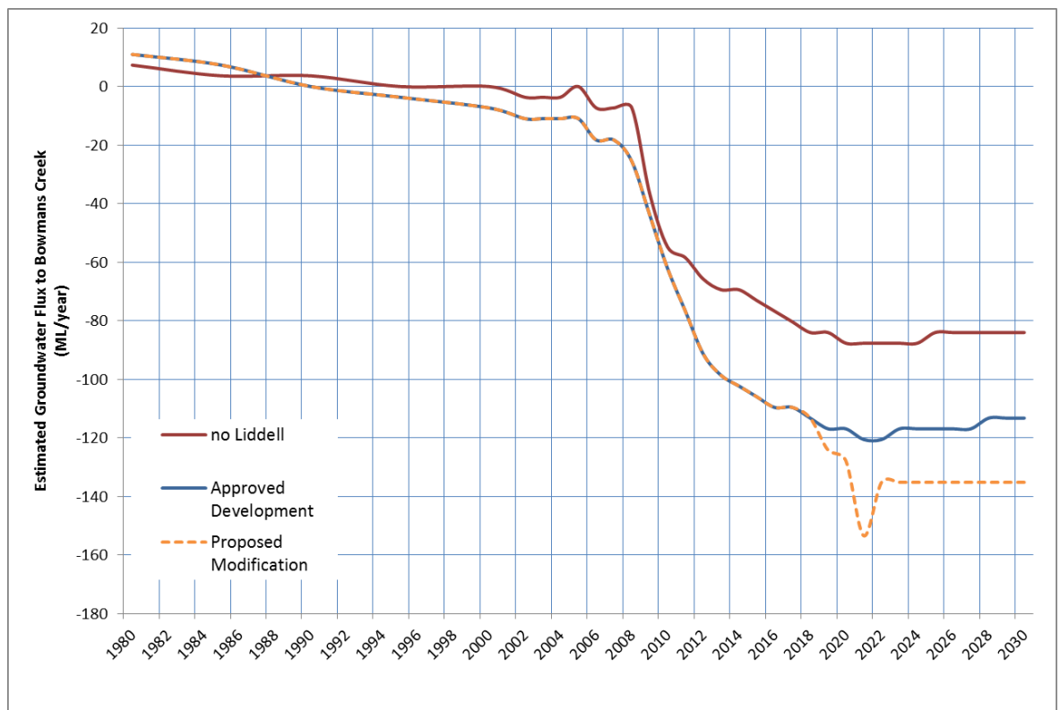
■ Figure 3-14 – Estimated Groundwater Flux to Bowmans Creek Alluvium
