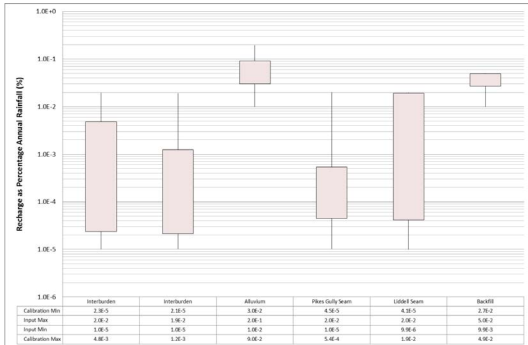
■ Figure 3-11 – Model Parameter Sensitivity: Recharge
