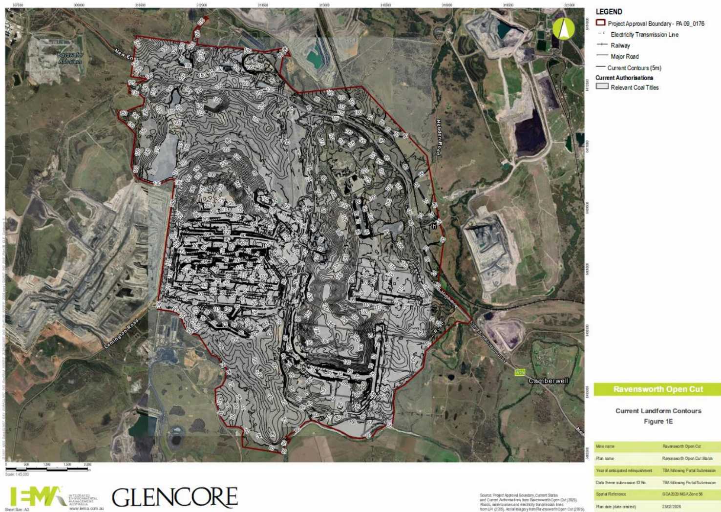
Figure 1E – Current Landform Contours
